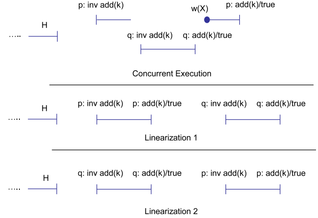
Figure 5. Illustration of the reasoning for why RAW is required in linearizable algorithms.
